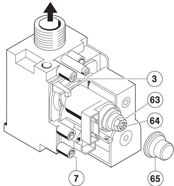
Fig. 52 Valvola gas
