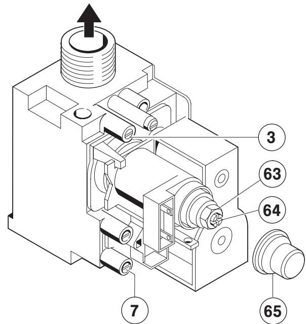
Fig. 50 Valvola gas
